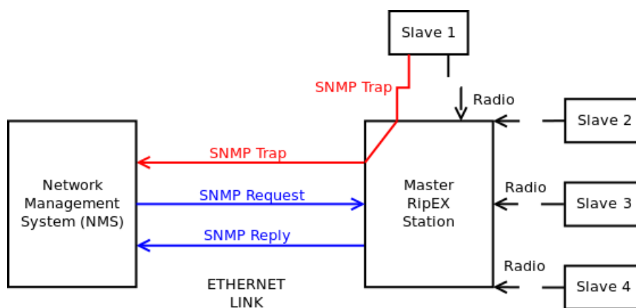
Fig. 2.2: NMS communication with Slave stations
