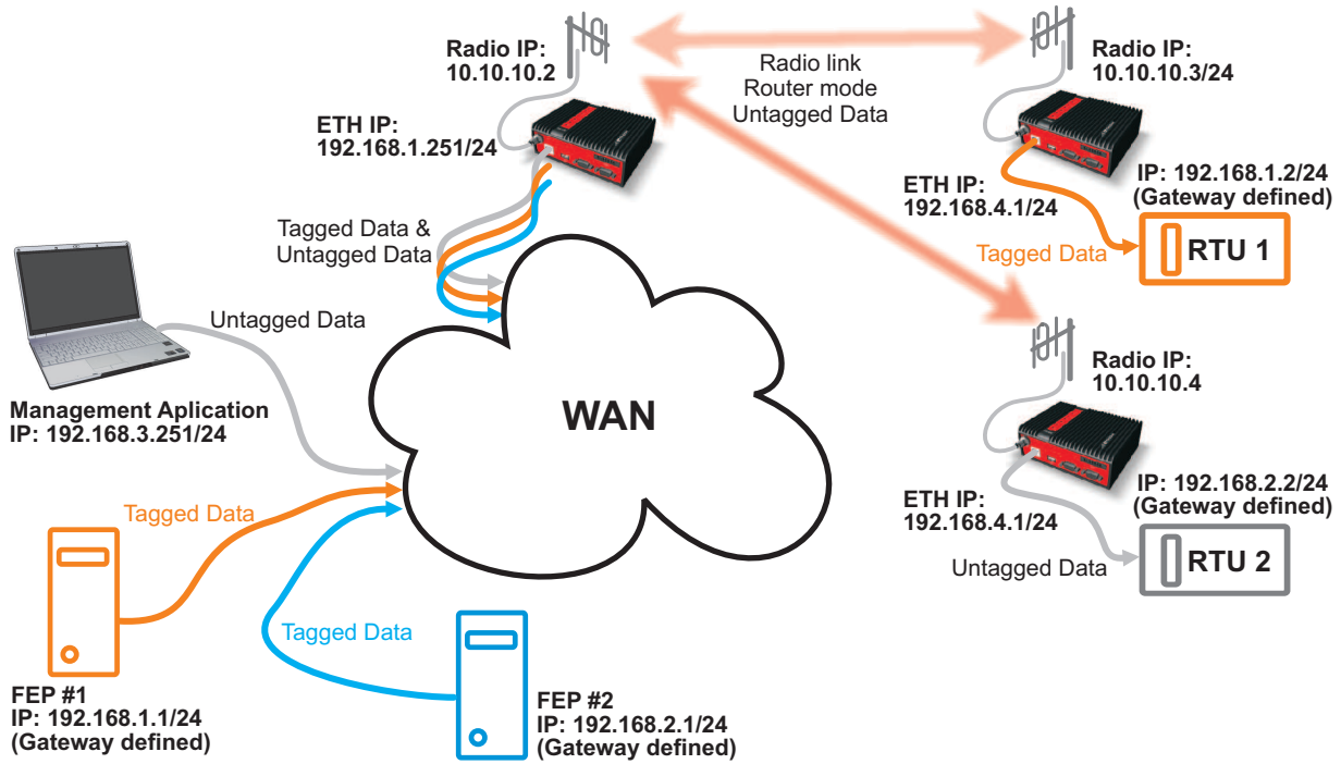
Fig. 11.2: VLAN diagram
