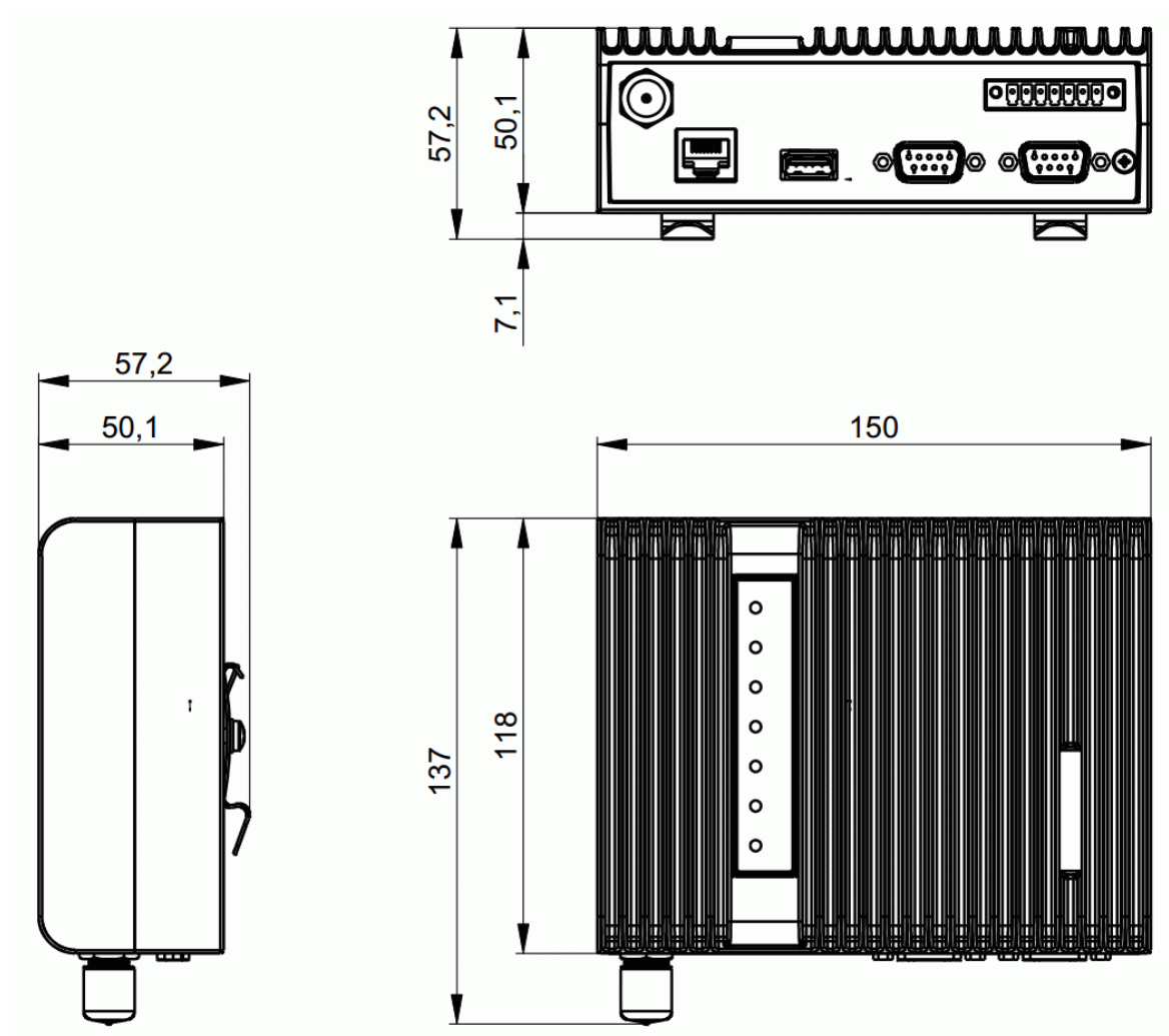
Fig. 5.1: RipEX dimensions
