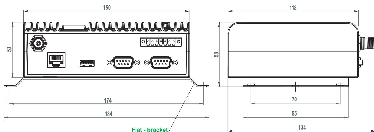
Fig. 5.21: RipEX with Flat-bracket
