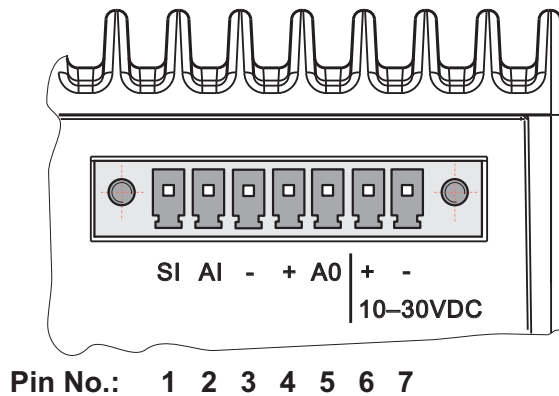
Fig. 5.8: Supply connector
