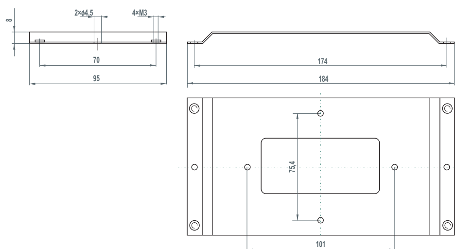
Fig. 5.22: Flat-bracket dimensions
