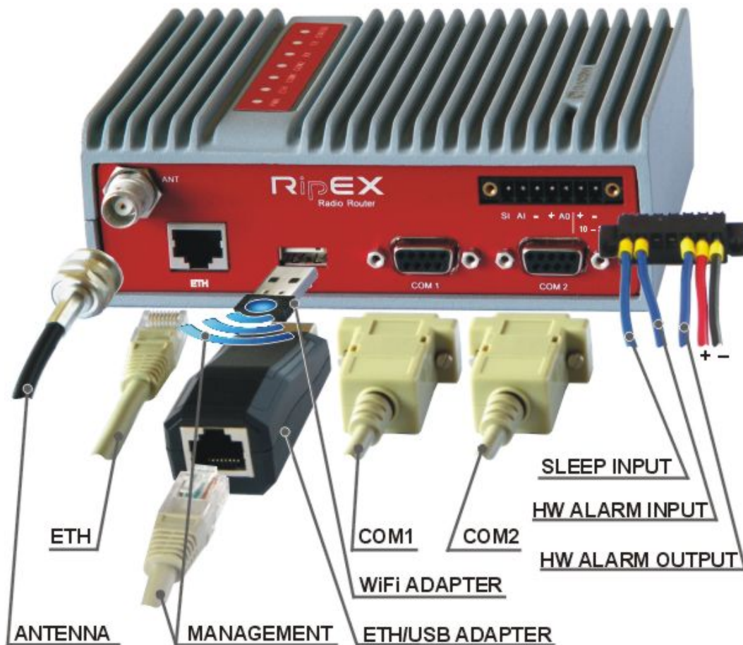
Fig. 5.5: Connectors
