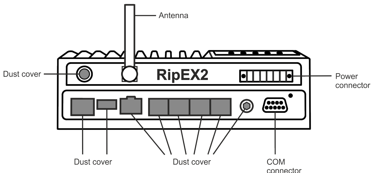
Fig. 4.8: IP5x protection
