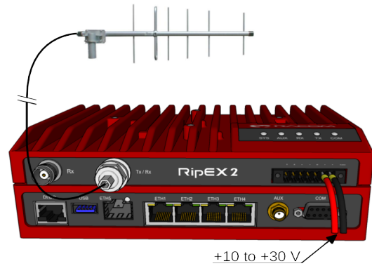
Fig. 4.10: 10–30 VDC Supplying
