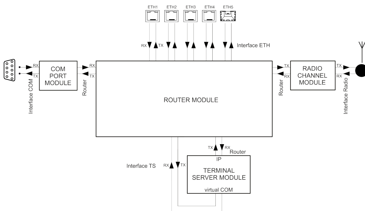
Fig. 8.2: Interfaces
