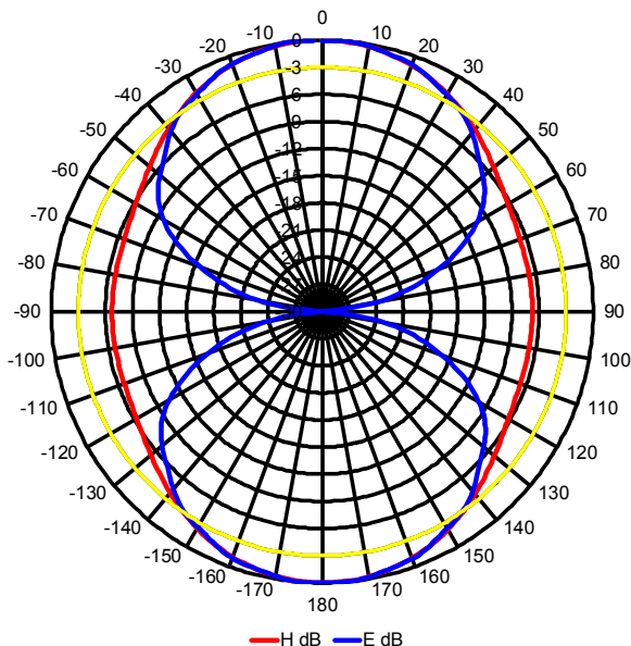
RADIATION PATTERN
