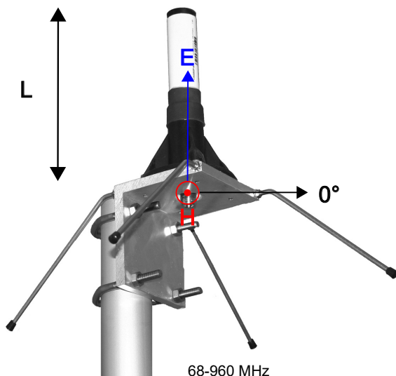
68-960 MHz
