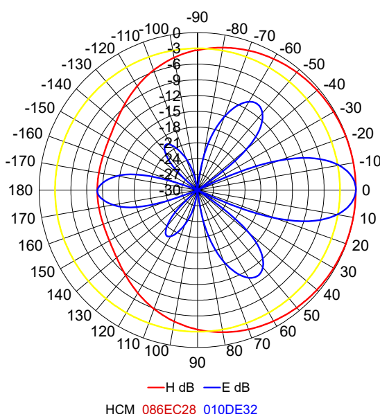
RADIATION PATTERN
