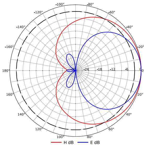
Radiation Pattern 892.5 MHz
