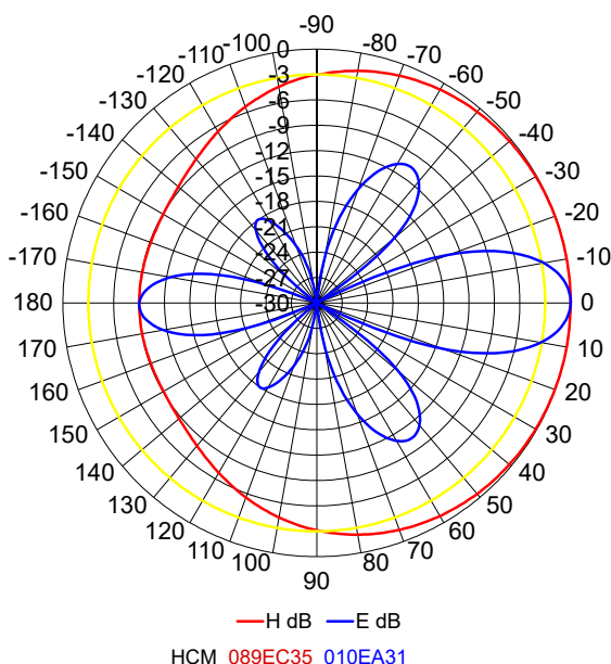
RADIATION PATTERN
