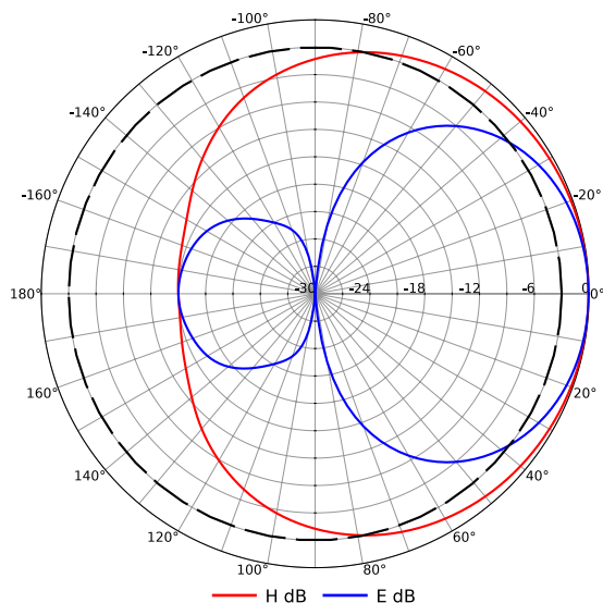
Radiation Pattern 757.5 MHz
