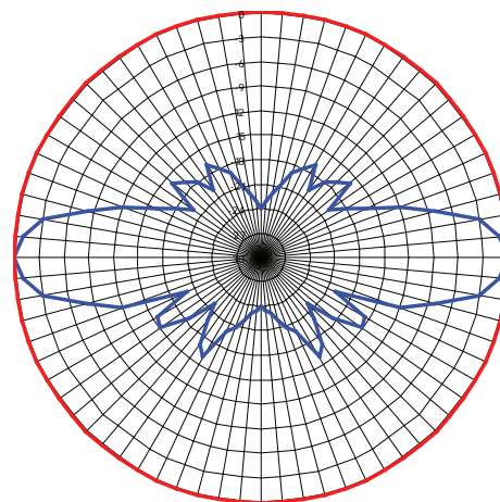
RADIATION PATTERN
